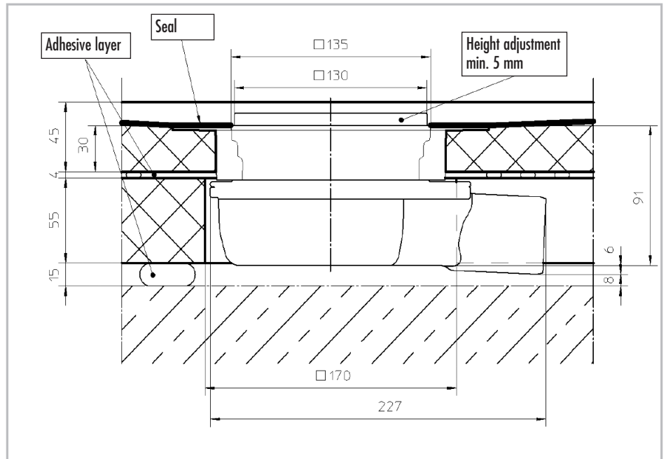
– DN 50 horizontal drain connection fitting with removable siphon trap
