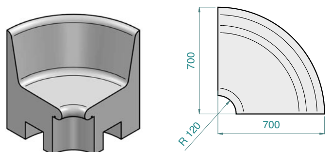
Corner round, bench + backrest – CONCEPT-BA ... ER-SL
