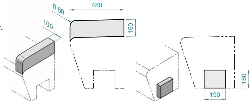
Bench end armrest – CONCEPT-BA ... AL
